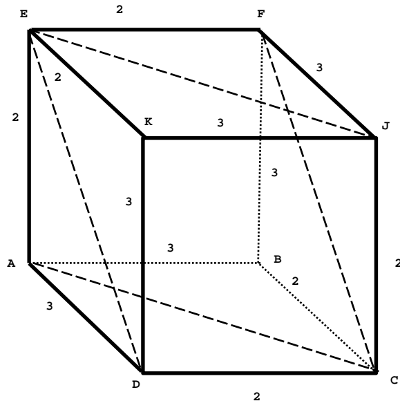
Figure 2: Symmetries of the hyperbolic polyhedron \Phi .
