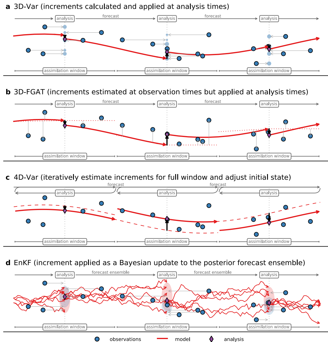
Figure 4. Simplified schematic representations of four data assimilation strategies used by current reanalyses: (a) 3D-Var, (b) 3D-FGAT, (c) incremental 4D-Var, and (d) EnKF. Blue circles represent observations, red lines represent model trajectories, and purple diamonds indicate analyses. The dotted red lines in (b) represent linearly interpolated/extrapolate forecast values used to estimate increments at observation times. The dashed red lines in (c) represent the initial forecast, prior to iterative adjustments. These illustrations are conceptual, and do not accurately reflect the much more complex strategies used by reanalysis systems.
