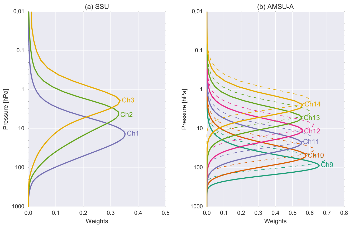
Figure 6. Vertical weighting functions of radiance measurements for (a) the TOVS-suite Stratospheric Sounding Unit (SSU) instrument (1979–2005) channel 1 (centred at ~15 hPa), channel 2 (~5 hPa), and channel 3 (~1.5 hPa), and (b) the ATOVS-suite Advanced Microwave Sounding Unit A (AMSU-A) instrument (1998–present) temperature channels 9–14 at near nadir (1.67°, solid lines) and limb (48.33°, dashed lines) scan positions. SSU channels 1 through 3 may also be referred to as TOVS channels 25 through 27.
