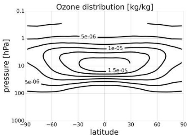
FIG. 2. Ozone distribution used in all simulations. MiMA reads ozone from an input file, which in our case contains a static and both zonally and north-south symmetric distribution based on the work of Fortuin and Langematz (1994). Contour interval is 2.5 ppm.
