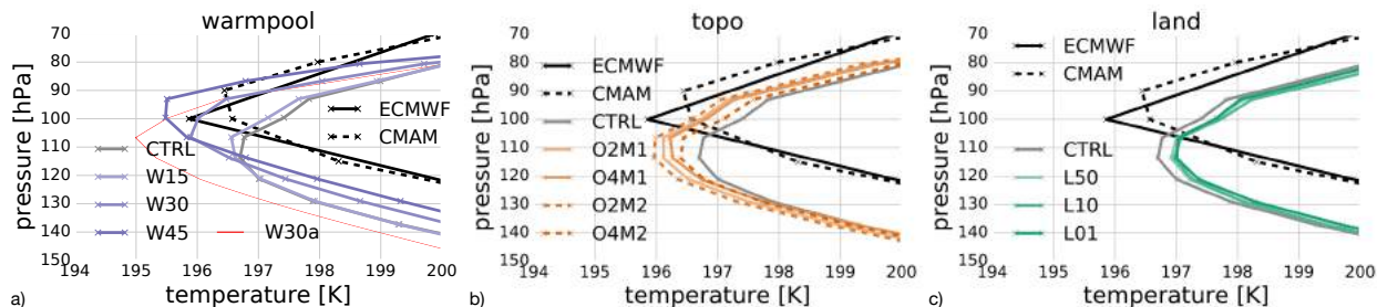
FIG. 4. Vertical temperature profiles of the tropical cold point region showing the effects of a) the tropical warm pool, b) midlatitude orographic forcing, and c) extratropical land-sea contrast on the annual mean cold point structure. Temperatures were averaged from 30^{\circ}\text{S} to 30^{\circ}\text{N} to construct the profiles. The tropical warm pool has the largest effect on the annual mean, whereas extratropical land-sea contrast has no effect in the mean. The fine red line in panel a) (labeled W30a) shows the temperature profile for W30 if the surface albedo is the same as in CTRL (see text for more discussion).
