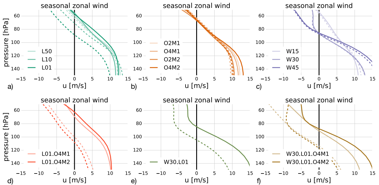
FIG. 12. Annual cycle of tropical zonal mean zonal wind profiles for parameter scans in a) midlatitude land-sea contrast, b) midlatitude topography, c) tropical warm pool, and the mixed cases d) land-sea contrast plus topography, e) tropical warm pool plus land-sea contrast, and f) tropical warm pool, land-sea contrast plus topography. Solid lines denote DJF, dashed lines JJA. The strength of the annual cycle in tropical zonal mean zonal wind profile is directly related to the strength of the annual cycle in temperature (Figures 7 and 8).
