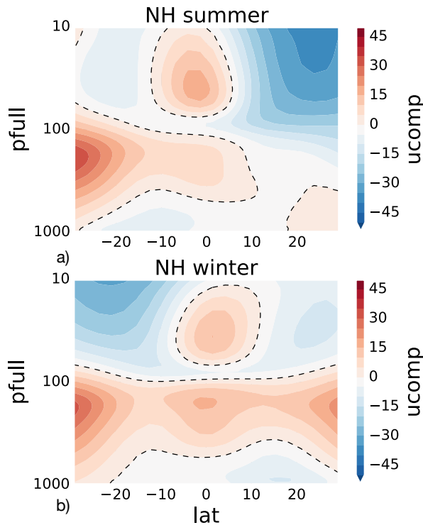
FIG. 11. Latitude-pressure contours of tropical zonal mean zonal wind in Northern Hemisphere Summer (top) and winter (bottom). The black dotted line denotes u = 0 , i.e. the critical line for stationary Rossby waves. Shows the case W30.L01.O4M2; this is the integration with the largest seasonal cycle.
