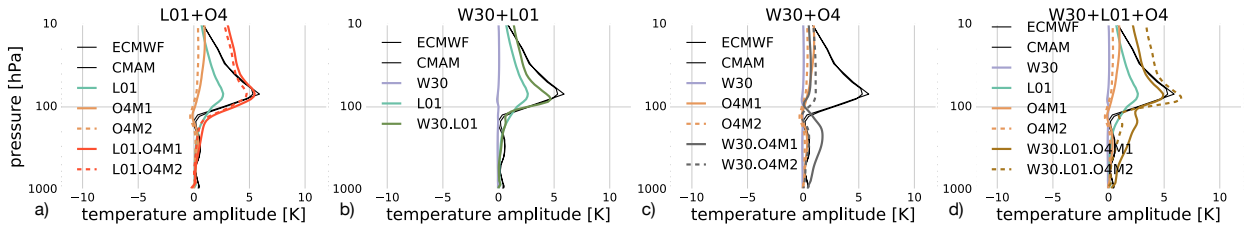
FIG. 8. Vertical profile of tropical temperature seasonal cycle ( 30^{\circ}\text{S} to 30^{\circ}\text{N} ) as in Figure 7, but for mixed parameter scans of a) midlatitude land-sea contrast and topography, b) midlatitude land-sea contrast and tropical warm pool, c) tropical warm pool and midlatitude topography, and d) tropical warm pool, midlatitude land-sea contrast and topography. Adding topography or a tropical warm pool to land-sea contrast more than doubles the seasonal cycle, even though topography itself does not have a strong influence, and the warm pool has no effect by itself. Indeed, only adding those two forcings together (panel c)) does not have any significant effect on the TTL annual cycle. Adding all three forcings together has the strongest effect, and the forcing case with tropical warm pool, land-sea contrast, and wave-two topography ( W30.L01.O4M2 ) even surpasses the annual cycle in reanalysis (dotted brown line in panel d)).
