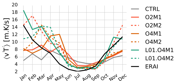
FIG. 5. Seasonal variation of meridional heat flux \langle v'T' \rangle at 100 hPa and averaged 30^{\circ}\text{--}90^{\circ}\text{N} . The addition of 4 km wave-two Gaussian mountains in midlatitudes allows for a very realistic variation in stationary wave forcing when compared to ERA-Interim. Adding land-sea contrast enhances the seasonal cycle even further.
