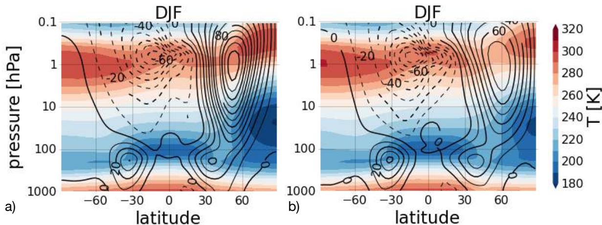
FIG. 1. Control climatological DJF zonal mean zonal wind (contours, interval 10 m/s) and temperature (shading). The control run (a) is north-south symmetric, with a uniform slab ocean with mixed layer depth 100 m (CTRL in Table 1). For comparison, panel (b) shows the DJF climatology of a simulation with wave-one 4 km topography and 1 m midlatitude ‘land’ (L01.O4M1 in Table 1). The polar vortex weakens by about 40% when adding this additional forcing in the NH midlatitudes.
