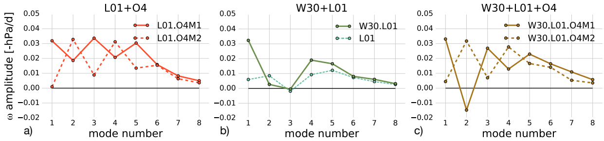
FIG. 10. Annual cycle of tropical upwelling decomposed into wave numbers for the three cases with the largest annual cycle in temperature. Even though the temperature response in Figure 8 suggests nonlinear interactions, upwelling still is a combination of the forcings: a) synoptic waves plus uneven (even) wave numbers for L01+O4M1(M2). b) clear separation between wave-one tropical and synoptic extratropical forcing. c) W30+L01+O4M2 is very similar to L01+O4M2 plus a small increase in wave-one forcing, whereas W30+L01+O4M1 shows a much more complex behavior, with wave-two even counteracting tropical upwelling.
