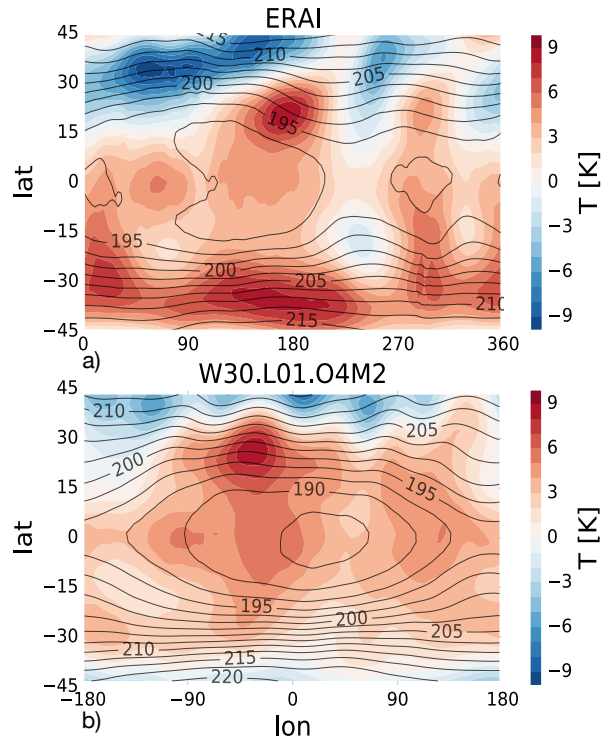
FIG. 9. Longitude-latitude contours of annual mean temperature (contours) and seasonal cycle (shading) at 100 hPa. (top) ERA-Interim and (bottom) MiMA. Note the strong similarities in structure, and in particular the localized maximum just off the cold point.
