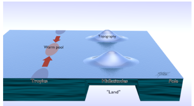
FIG. 3. The three key surface forcings used to modulate the TTL in MiMA. Extratropical planetary waves are excited by Gaussian-shaped mountains positioned in the midlatitudes. Tropical planetary waves are excited by a purely zonal heat flux within the tropics, which generates a ‘warm pool’ (i.e. a localized region of maximum SSTs along the equator) that in turn drives zonal asymmetry the tropical convection. Lastly, synoptic variability is modulated by reducing the heat capacity of the mixed layer ocean in the midlatitudes of one hemisphere, a very crude approximation to ‘land’ which in turn amplifies the annual cycle of midlatitude baroclinicity.
