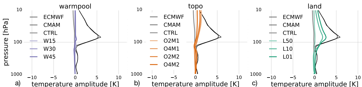
FIG. 7. Vertical profile of the tropical temperature seasonal cycle (June–July–August mean minus the December–January–February mean, averaged from 30^{\circ}\text{S} to 30^{\circ}\text{N} ) for single parameter scans of a) tropical warm pool strength, b) midlatitude topography, and c) midlatitude ‘land’ mixed layer depth. Mixed layer depth is labeled LD , where D is the mixed layer depth in meters ( D = 100 m for CTRL). Topography is labeled OHMm , where H is the height in km, and m the wave number ( H = 0 km for CTRL). Warm pool strength is labeled WQ , where Q is the zonal heat flux in \text{W}/\text{m}^2 ( Q = 0 \text{W}/\text{m}^2 for CTRL). As expected, the tropical warm pool does not induce a seasonal cycle, as there is no North–South asymmetry in the forcing. Topography does create a seasonal cycle, but mostly in the upper stratosphere, and the profile is qualitatively very different to reanalysis. In contrast, midlatitude land–sea contrast (‘land’) has an effect which is qualitatively correct, though somewhat weak.
