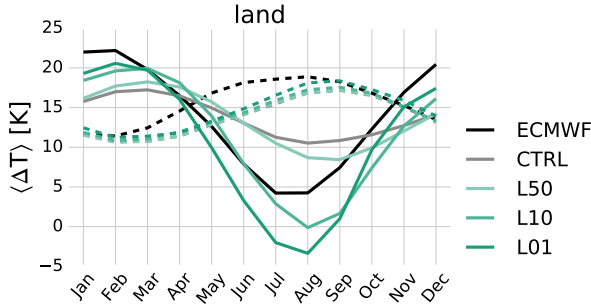
FIG. 6. The monthly variation of the temperature difference between the equator and 45°N(S) for continuous (dotted) lines, averaged over the depth of the troposphere (1000 to 250 hPa). The mixed layer in CTRL is everywhere equivalent to 100 m of sea water, but reduced to 50, 10, and 1 m depth between 40 and 50°N in the integrations L50, L10, and L01, respectively.
