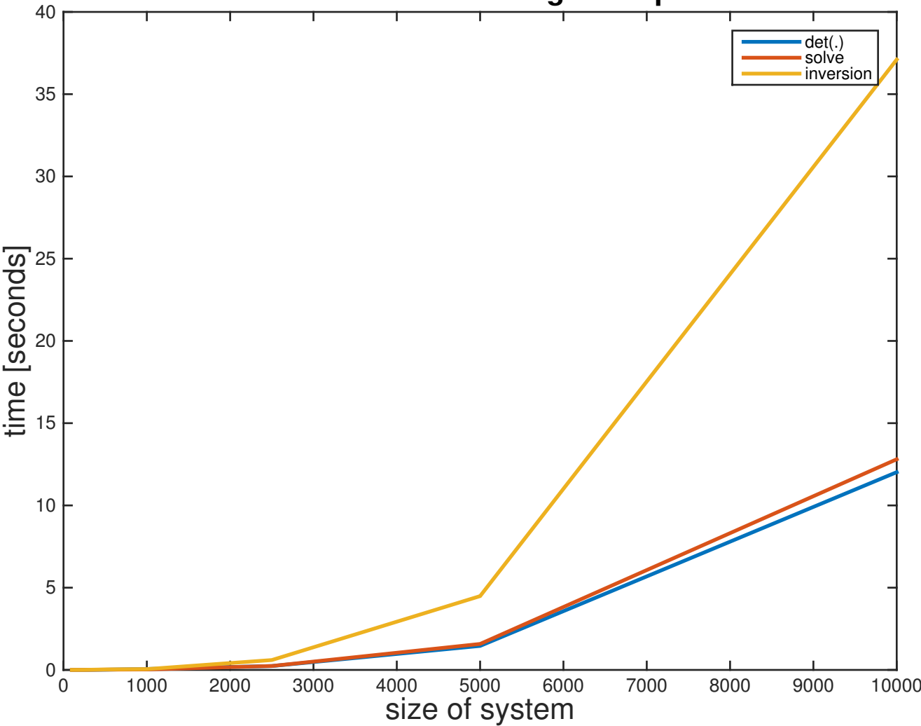
times for different linear algebra operations
