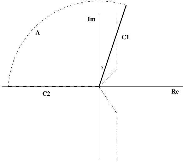
Rotation of the integration contour to the real axis
