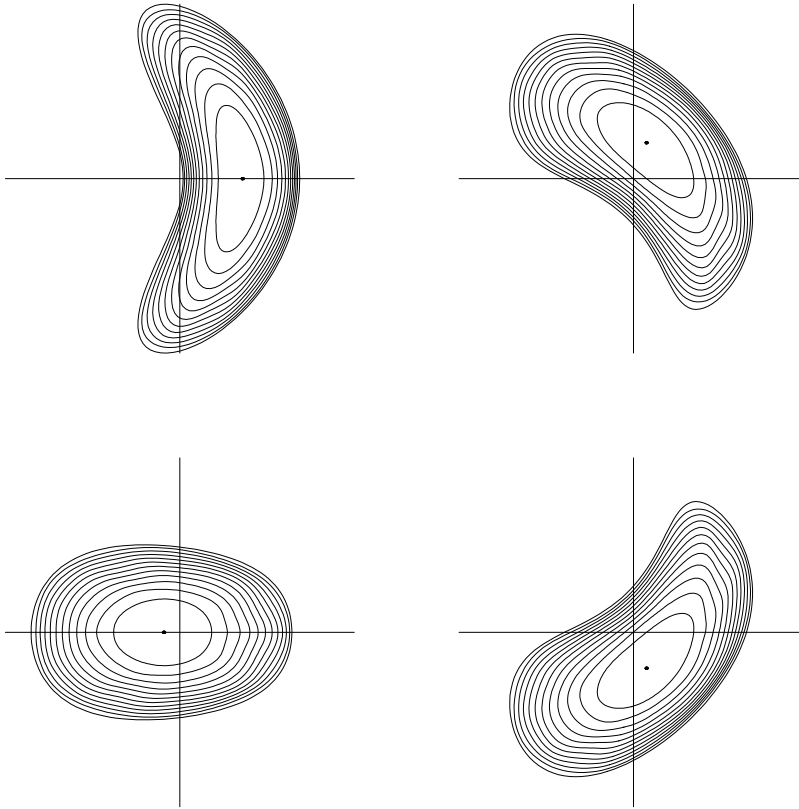
Figure 1: Flux surfaces at four cross sections over the two field periods of a stellarator equilibrium at \beta = 0.03 . The rotational transform \iota increases from the low value 0.33 at the magnetic axis to a peak value of 0.47 and then falls to 0.40 at the separatrix. This configuration is a good candidate for DEMO because its geometry is similar to that of the ITER tokamak. There is enough flexibility in the shaping of the plasma to control the stellarator contribution to \iota so as to compensate for unforeseen complications with the bootstrap current.
