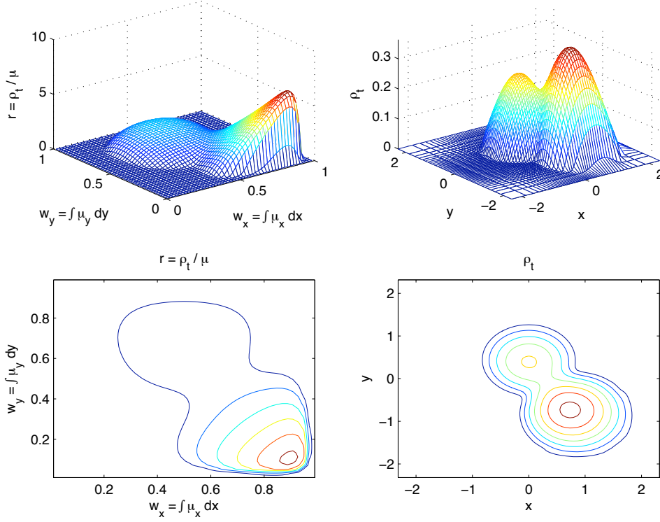
FIG. 3.3. Same as in figure 3.2 at time t=0.5 .
