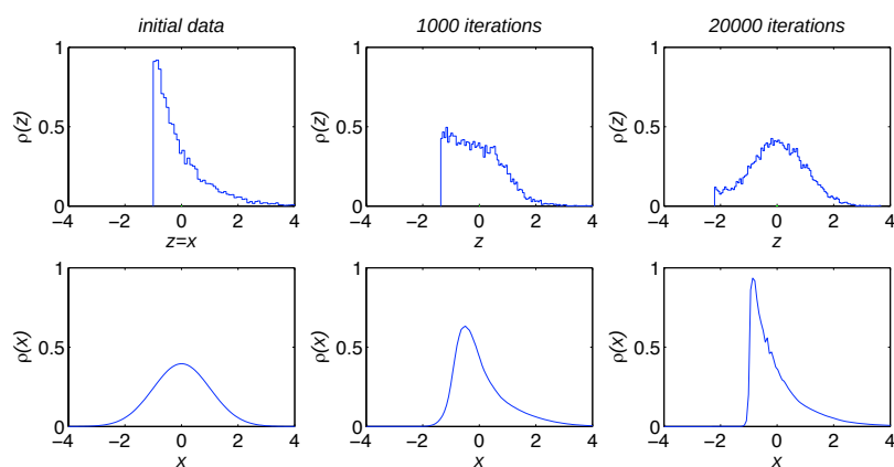
FIG. 7.1. Illustration of the algorithm on a sample drawn from a one-dimensional centered exponential density. The top panels show the evolution of the empirical distribution toward the target Gaussian. The bottom panels show the dual evolution of the density of the original sample as estimated by the procedure. Note that, as the empirical density evolves from the exponential toward the Gaussian, the estimated density evolves from the Gaussian toward the exponential.
