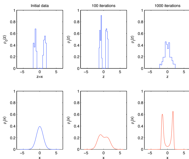
FIG. 7.2. Same as in figure 7.1 for a sample drawn from a distribution uniform on two intervals. In this figure, the number of data point is 200 only. This explains why the density produced by the procedure is not as sharply separated into two as the original density. The quality of the estimated density improves with the number of sampled points, as illustrated in figure 7.3.
