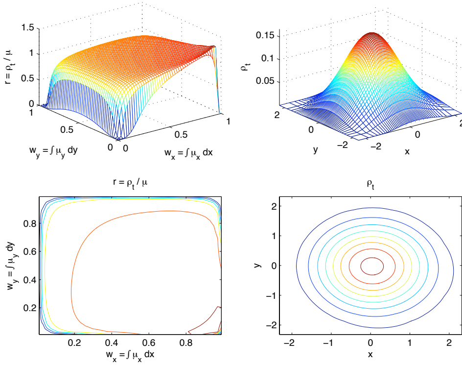
FIG. 3.4. Same as in figure 3.2 at time t=20 .
