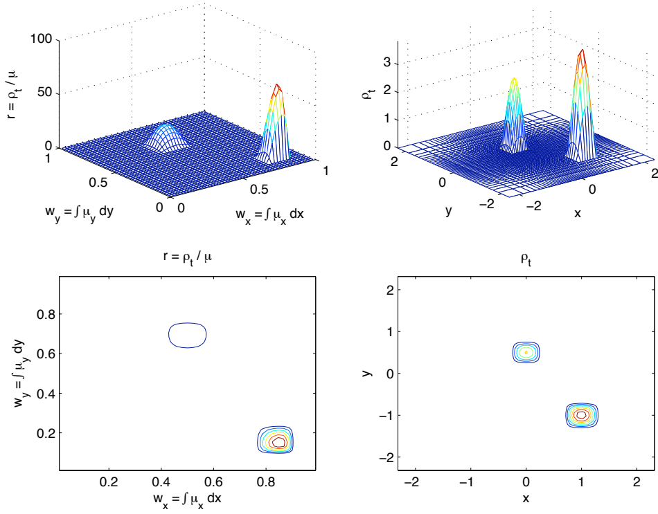
FIG. 3.2. Numerical solution of (3.6) for the two dimensional example of the density made of the superposition of two bumps described in text. The left panel shows r_t as a function of (w_x, w_y) at time t=0 ; the right panel shows the corresponding \rho_t as a function of (x, y) .
