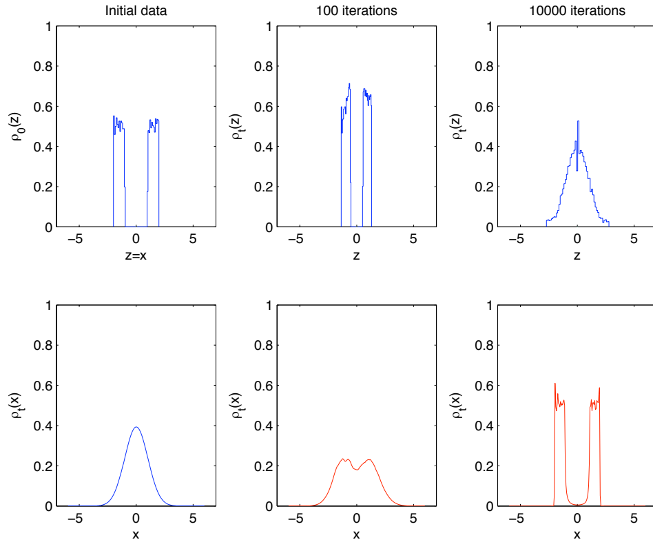
FIG. 7.3. Same as in figure 7.2 but with a sample containing 10000 points. Note that the two modes of the density are much better separated than in figure 7.2.
