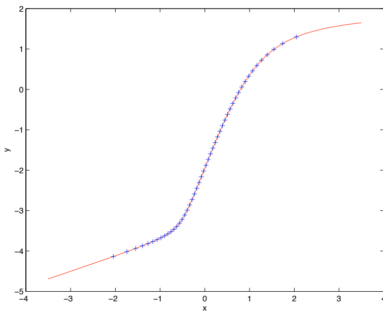
FIG. 6.1. The solid curve shows the result of the successive application of two maps (6.1) on the identity function. The crosses are points on a equiprobability grid of a Gaussian distribution. Notice that the choice of mollifier \epsilon in (6.2) guarantees that the smaller the density of crosses, the more aggressive the mollification of the map.
