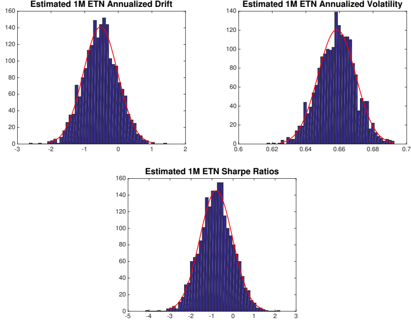
Figure 11: Top Left: The histogram of estimated drifts for the simulated 1M ETNs. Historically, the 1M ETN VXX recorded an estimated drift of \hat{m} = \frac{1}{N\Delta t} \sum_{\ell} \frac{\Delta VXX_{t_{\ell}}}{VXX_{t_{\ell}}} = -.6418 between 3/1/2010 and 3/1/2017, which is within the bulk among simulated drift estimators. Top Right: For the same time period the historically estimated volatility for the VXX was \hat{s} = \sqrt{\frac{1}{N\Delta t} \sum_{\ell} (\Delta \ln(VXX_{t_{\ell}}) - \overline{\Delta \ln(VXX)})^2} = 0.6301 , which is at the edge of the bulk among simulated volatility estimators. Bottom: The historically estimated VXX Sharpe ratio \hat{m}/\hat{s} = -1.0185 , which is within the bulk among simulated Sharpe ratio estimates.
