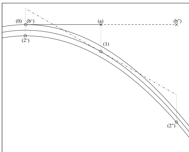
Figure 3. Delta-hedging with a concave value-function, with A < 1 . The curves corresponding to different time-sections of the value function increase with time. The greatest risk is when then the price goes up and then goes down. If delta-hedging is used, the position goes from (0) to (1) to (2). With a static hedge, the value of the portfolio goes from (0) to (a) to (b), and hence falls below the theoretical value.
