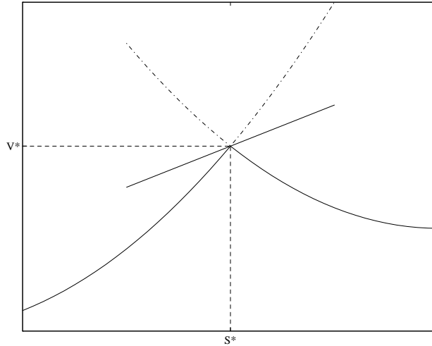
Figure 5. Schematic rendering of a function V(S, t) with a “locally concave” kink. The straight line segment through the kink lies above the graph of the function. Therefore, if the price of the underlying is S^* , the initial value of a portfolio is V^* , and the number of shares is equal to the slope of the line segment, then a static strategy yields a value of the portfolio greater than V(S_t, t) , if the price remains in a neighborhood of S^* .
