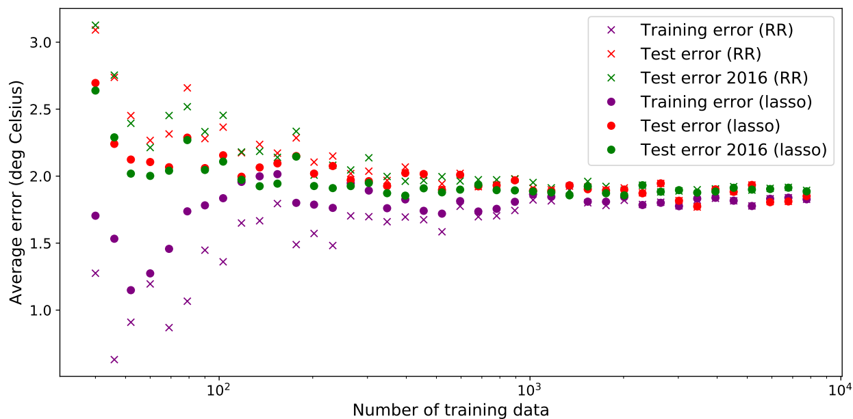
Figure 5: Performance of the lasso estimator on the temperature data described in Example 3.2. The graph shows the RMSE achieved by the models on the training and test sets, and on the 2016 data, for different number of training data and compares it to the RMSE achieved by ridge regression.
