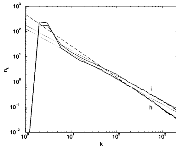
Fig. 10. Transition (h → i) from the MMT regime to the WT direct cascade (focusing nonlinearity with \alpha = \frac{1}{2} , \sigma = 0 ). The system is driven by a random force at 2 \leq |k| \leq 3 with a weaker strength than that in Fig. 9. There is damping at |k| = 1 and |k| > 2600 with the same damping strength as the case shown in Fig. 8. The slope of the dashed (dotted) line is the prediction of the MMT (WT) closure.
