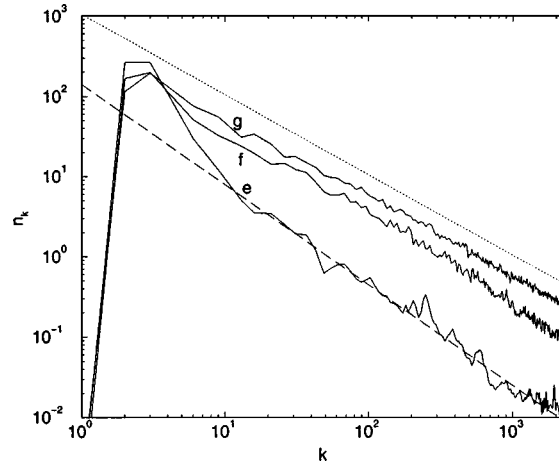
Fig. 9. Transition (e → g) from the MMT regime to the WT direct cascade (focusing nonlinearity with \alpha = \frac{1}{2} , \sigma = 0 ). The system is driven by a random force at 2 \leq |k| \leq 3 with a weaker strength than that in Fig. 8. There is damping at |k| = 1 and |k| > 2600 , with the same damping strength as the case shown in Fig. 8. The slope of the dashed (dotted) line is the prediction of the MMT (WT) closure.
