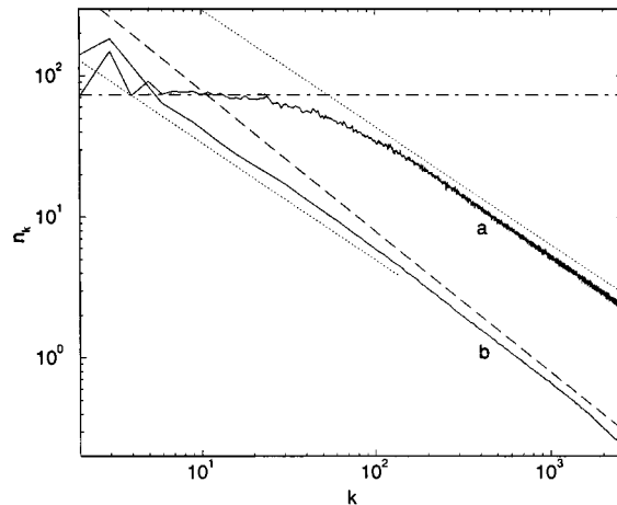
Fig. 19. (a) Coexistence of thermodynamical equilibrium and the inverse WT cascade, for the focusing nonlinearity ( \alpha = \frac{1}{2}, \sigma = 0 ), driven by a steady force on |k| = 1 . The flat part of the spectrum (dot-dashed line) shows thermodynamical equilibrium. (b) Coexistence of the inverse and direct WT cascades. The dotted (dashed) line has the exponent of inverse (direct) WT cascade.
