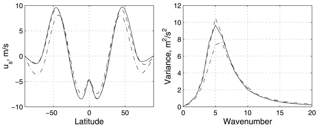
FIG. 2. (left) Resolution dependence of time mean zonal mean surface zonal winds. (right) Resolution dependence of zonal wavenumber spectra for \langle v \rangle at 45^\circ latitude. T170 (solid), T85 (dashed), and T42 (dash-dot).
