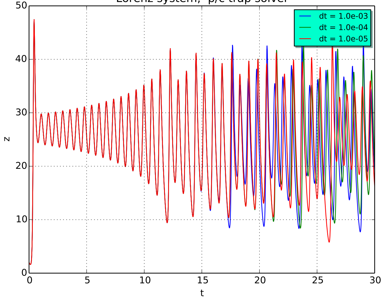
Lorenz system, p/c trap solver
