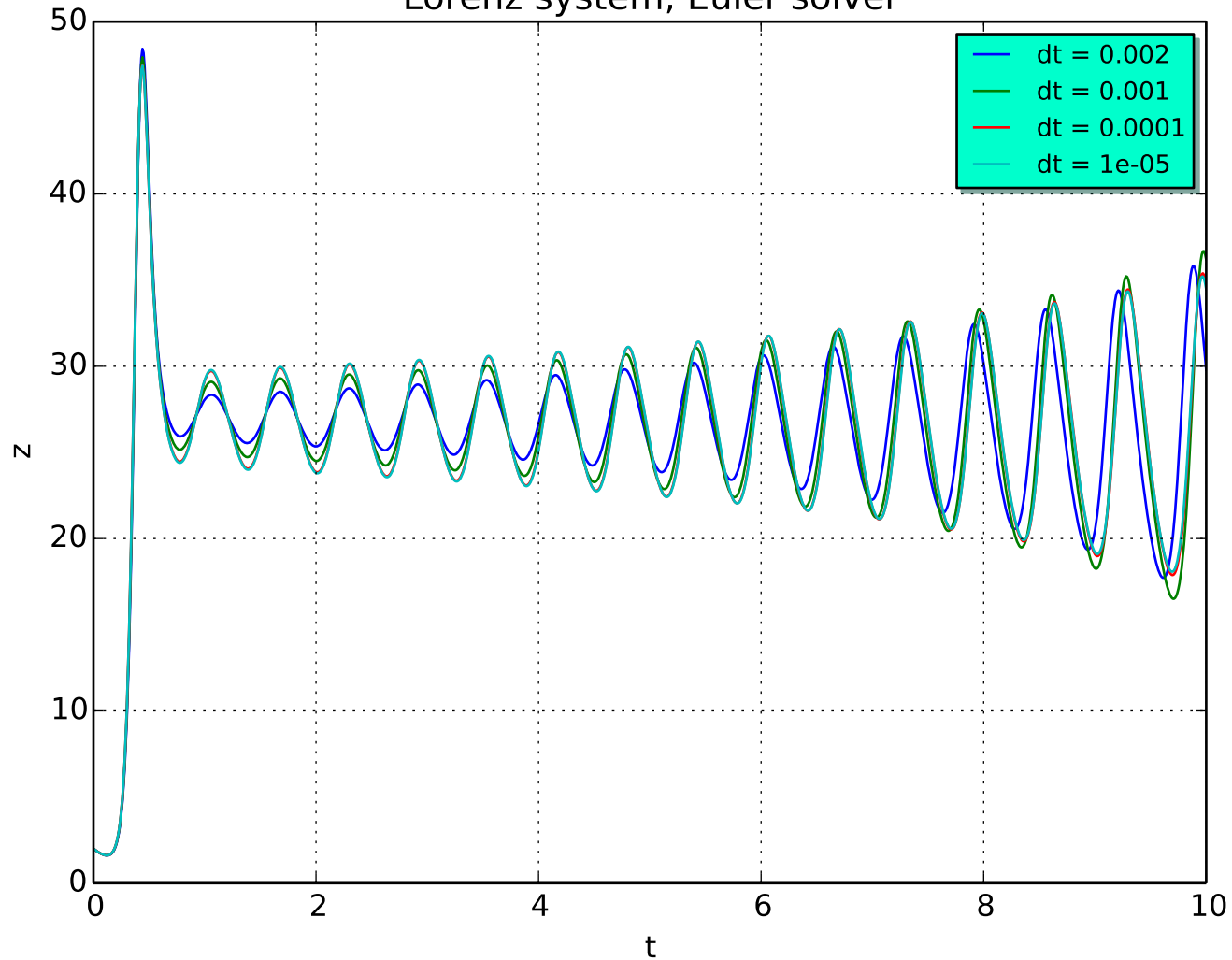
Lorenz system, Euler solver
