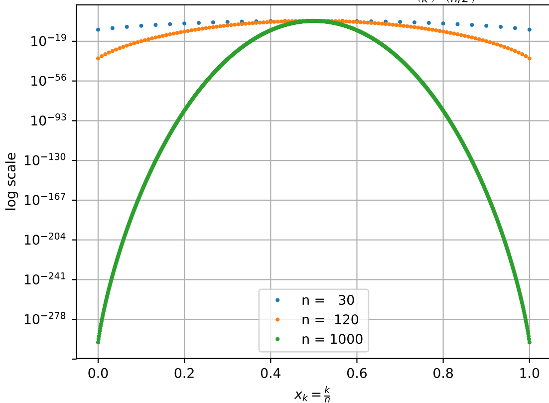
Normalized binomial coefficients \binom{n}{k} / \binom{n}{n/2}
