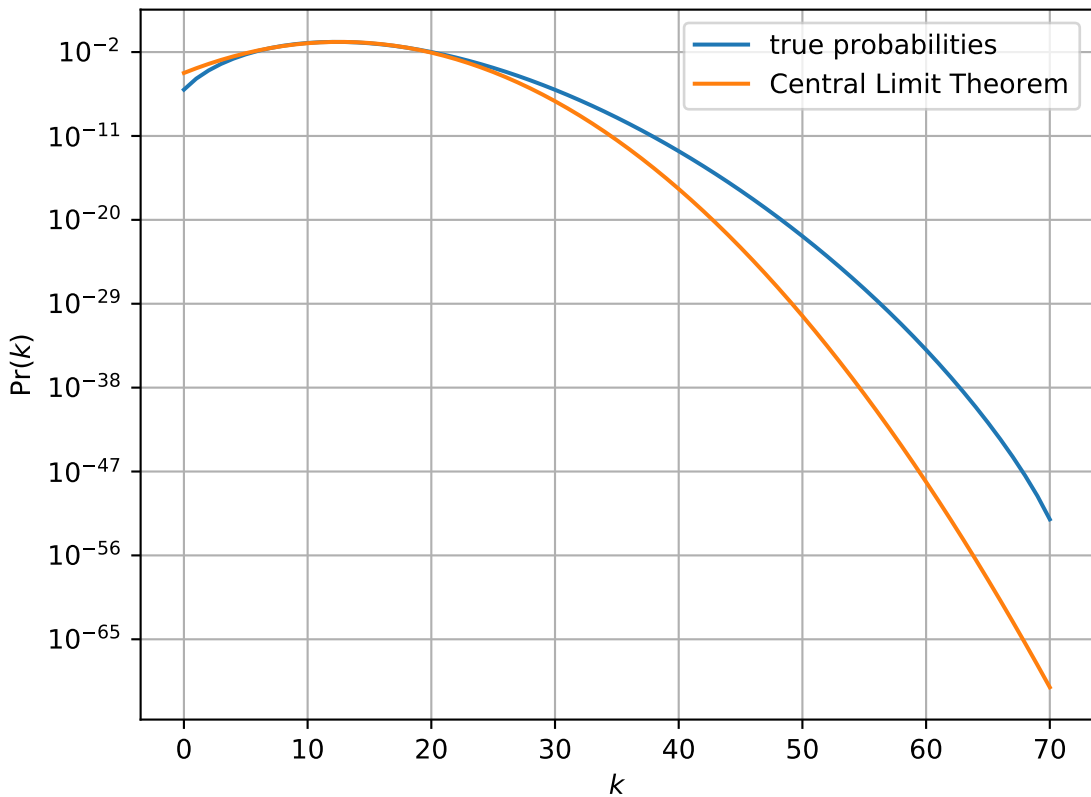
Binomial and CLT, whole range, log scale n = 70 , p = 0.18
