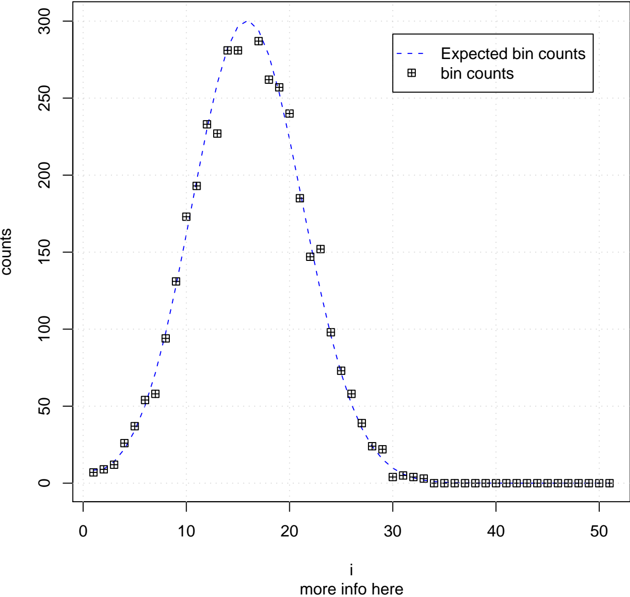
Histogram, urn process, 4000 paths, 50 steps, p = 0.30
