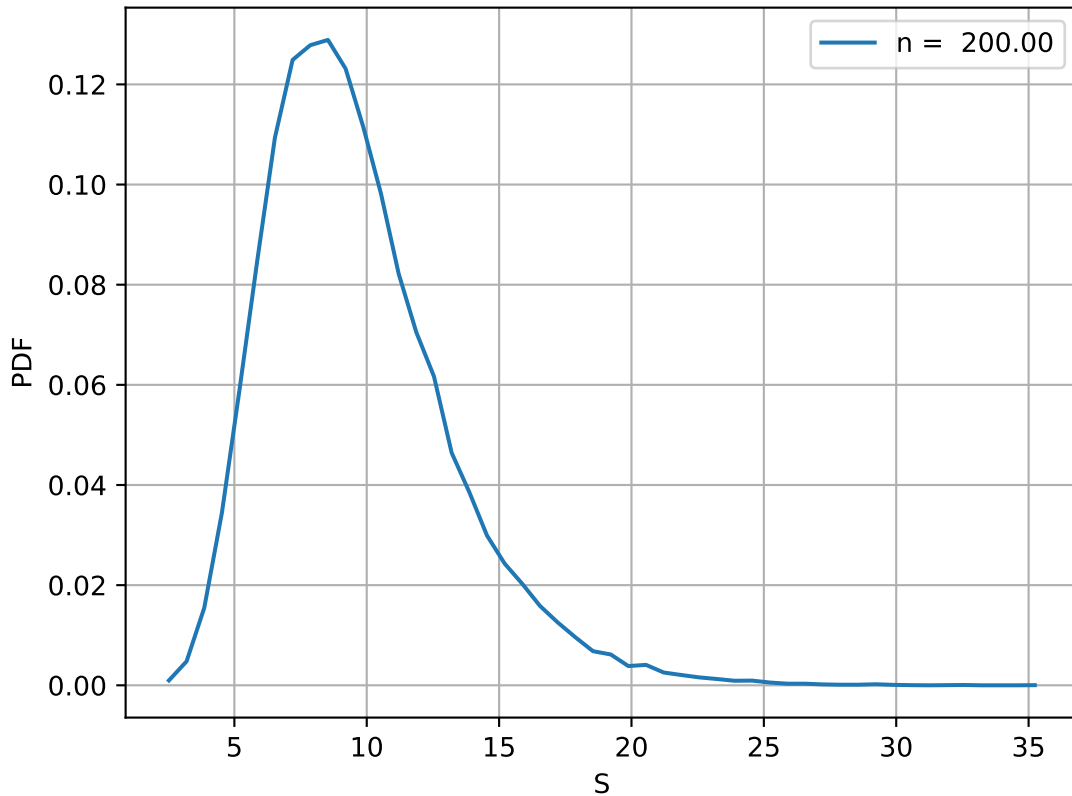
Final price PDF, T = 0.05 , \mu = 0.30 , \text{sig} = 1.50
