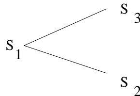
Figure 1: Prices in the one-period binomial market model.
