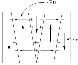
Figure 25: Charges in the bulk
