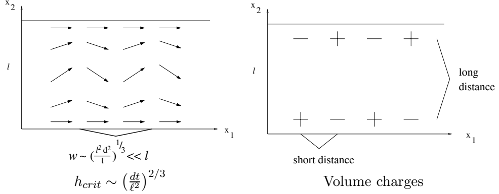
Figure 32: Oscillation
