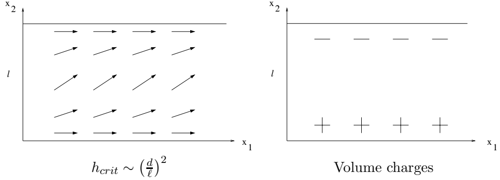
Figure 31: Buckling
