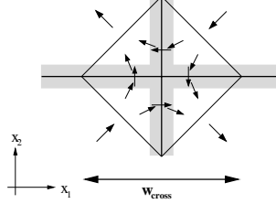
Figure 20: Winding Néel walls in cross-tie
