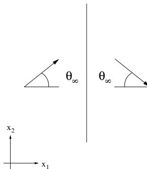
Figure 10: The wall angle \theta_\infty
