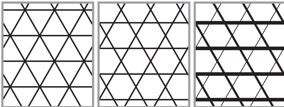
Fig. 1. In 2D, a triangular lattice (left) and a Kagomé lattice (center) are both examples of single-scale laminates; since they have the same layer directions and thicknesses, the Superposition Principle shows they have the same Hooke’s law. For a general single-scale laminate, the thicknesses of the layers can depend on their orientation; thus the structure shown on the right is also a 2D single-scale laminate.
