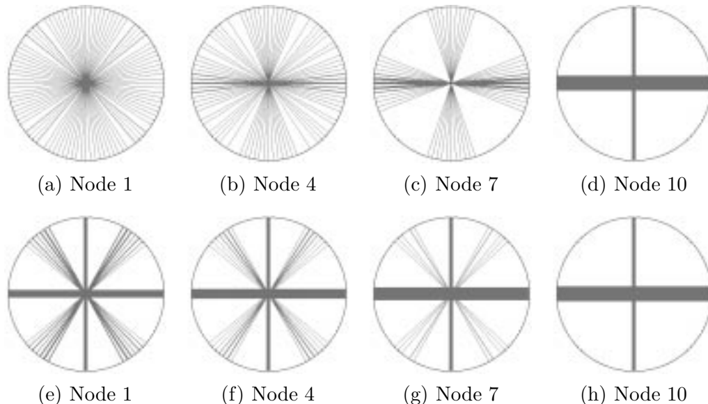
Fig. 3. Selection of single-scale laminates, when the Hooke's law varies linearly between an isotropic law and an orthotropic one. Top row: outcome of the semidefinite program from Section 4.1. Bottom row: outcome of the quadratic program (19).
