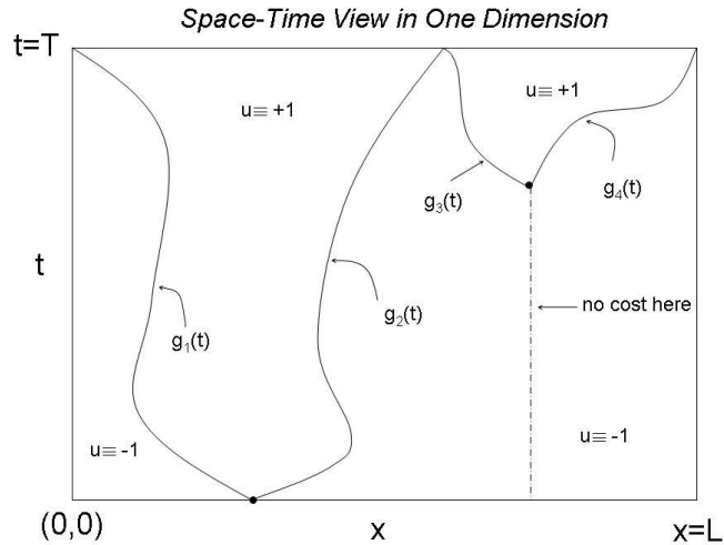
Figure 2: A space-time view of the sharp-interface limit of a switching path in one dimension. There are two nucleation events and the interfaces propagate in order to achieve switching by the switching time, t = T .
