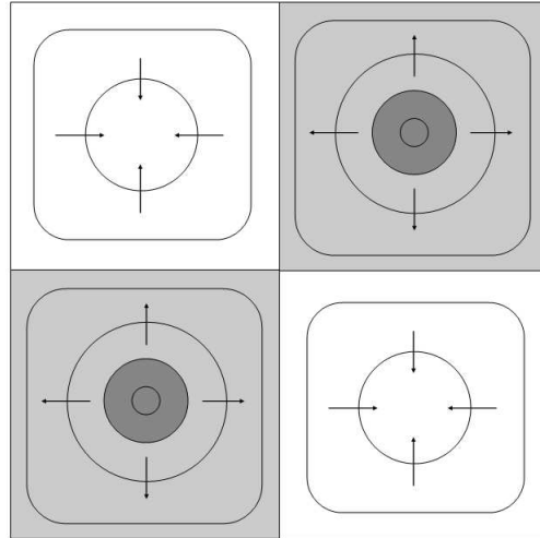
Figure 5: Sketch of an MCF construction. Reverse curvature motion carries the interface from two point nucleations to two gray squares. After the checkerboard is complete, the white squares collapse by forward curvature flow.
