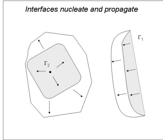
Figure 1: Interfaces forming and propagating in a two-dimensional system. The reduced action functional counts the perimeter of nucleated structures and the propagation cost of moving against curvature.
