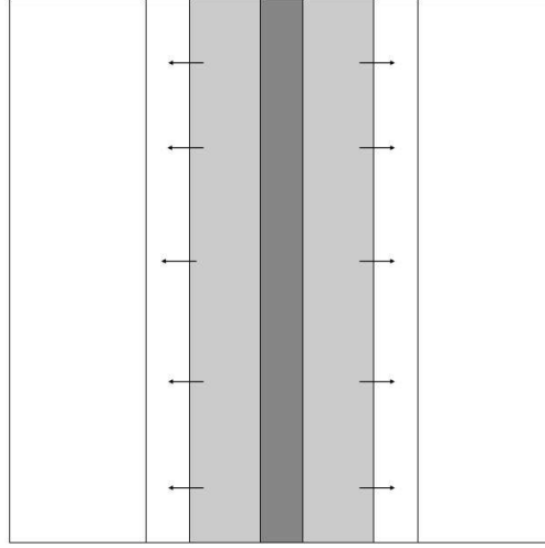
Figure 4: The stripe pattern, a one-dimensional construction for periodic boundary conditions.
