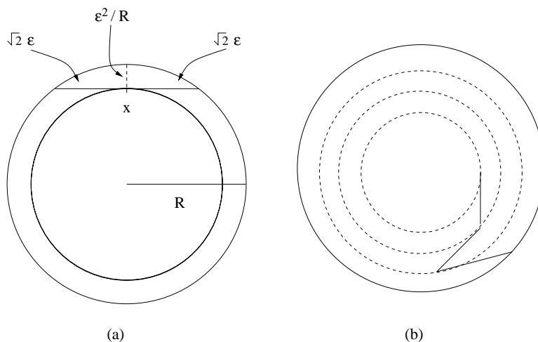
Figure 1: (a) If Paul starts close enough to the boundary, and he chooses v in the tangent direction, then he exits in one step no matter what Carol does. (b) If Paul starts farther from the boundary, his optimal strategy is to choose v at each stage tangent to the associated circle.
