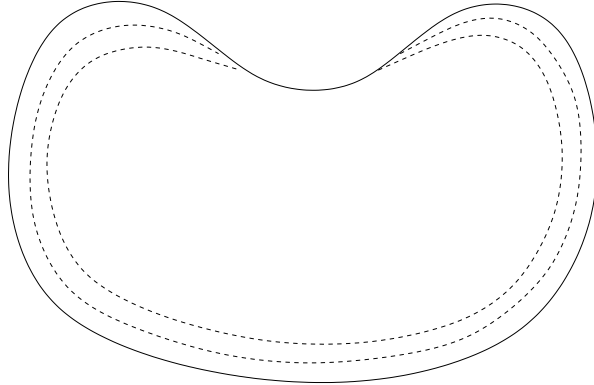
Figure 4: Schematic of motion by positive curvature for a nonconvex curve in the plane. The solid curve is the locus at a specific time; the dotted curves give the locus at two later times; we expect the “free boundary” separating the convex and concave parts to move along the solid curve.
