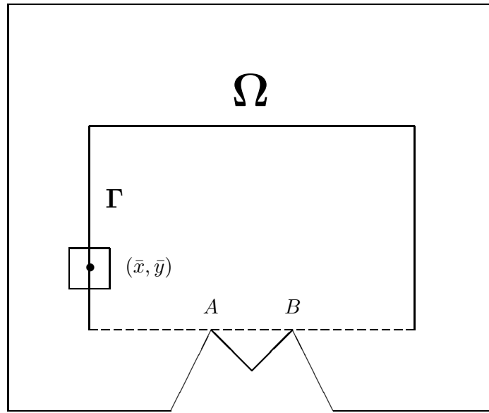
Figure 6: Paul’s limiting exit time is discontinuous at A and B . In fact, it vanishes along the segments joining A to B (and on the whole boundary), but it is bounded away from zero just above the dotted line.
