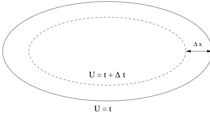
Figure 2: Level sets of U , the arrival time of the mean curvature flow.
