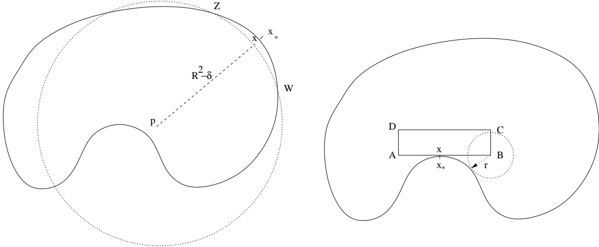
Figure 5: Left: The crescent-shaped region in the proof of (1.19). Right: the rectangle ABCD in the proof of (1.20).
