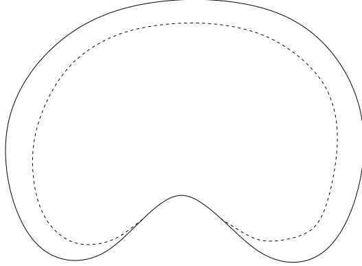
Figure 3: The dotted line consists of midpoints of segments of length 2\sqrt{2}\varepsilon with endpoints on \partial\Omega . If Paul starts on or outside it then he can exit in one step.
