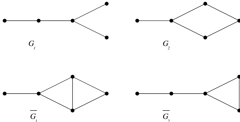
Figure 1: G_1 and G_2 have the Erdős-Hajnal property
