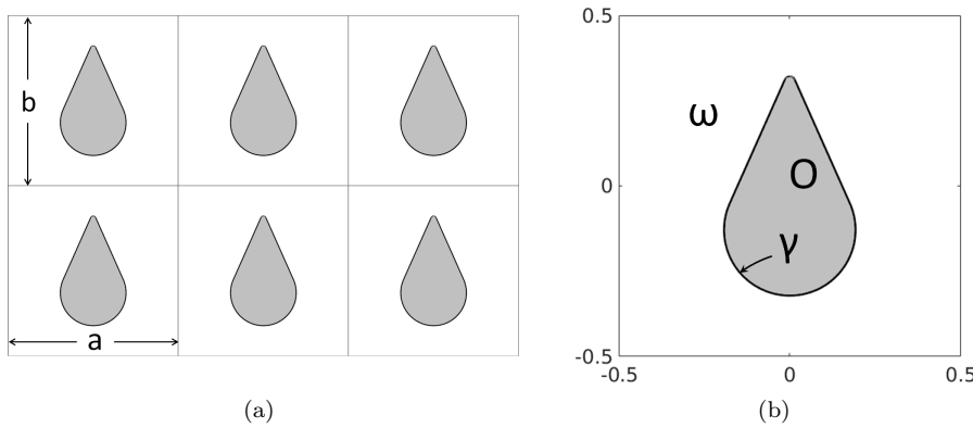
FIG. 2. (a) A periodic array of teardrop-shaped posts. Its unit cells, separated by solid lines, have width a and height b ; here a = b = 1 . Domains occupied by the posts are depicted as gray. (b) An enlarged view of one unit cell in (a). O denotes the gray domain occupied by the post; \omega denotes the exterior domain filled with fluid; \gamma denotes the boundary of \omega between them.
