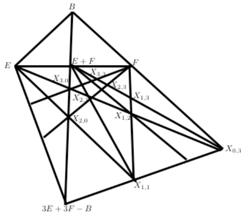
FIGURE 7. The stable base locus decomposition of \mathbb{F}_1^{[4]} .
